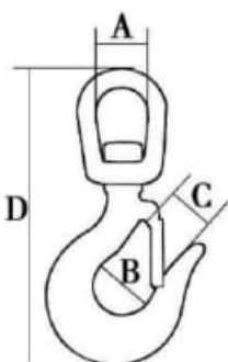
Sukamasis ąsa kranas kablys
