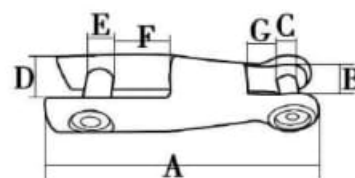
AISI316 STAINLESS STEEL ONE-PART ANCHOR SWIVEL CONNECTOR
