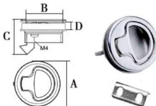
AISI316 STAINLESS STEEL ANGLE CODE LOCK BODY
