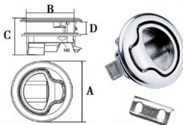
AISI316 STAINLESS STEEL TURNING LOCK LIFT HANDLE
