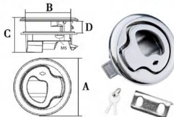
AISI316 STAINLESS STEEL TURNING LOCK LIFT HANDLE
